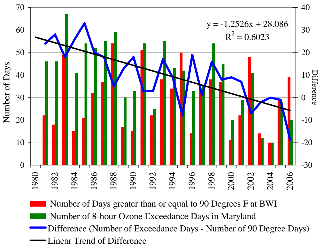
Figure 11.1.7 Improving air quality in Maryland is shown by the downward linear trend (black line) of the difference between (blue line) the number of 8-hour ozone exceedance days per year (green bars) and the number of days with a daily maximum temperature \geq 90^{\circ}\text{F} per year at BWI (red bars). The time period is 1981-2006.
