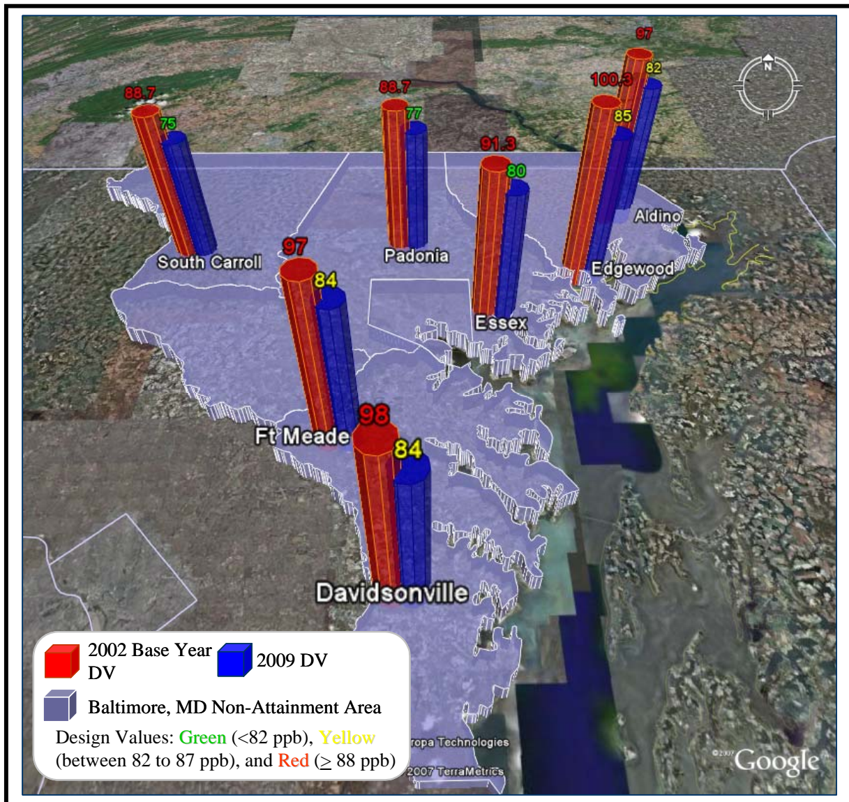
Figure 12-3 Baltimore NAA 8-Hour Ozone Base Year (2002) and Future Year (2009) Design Values
