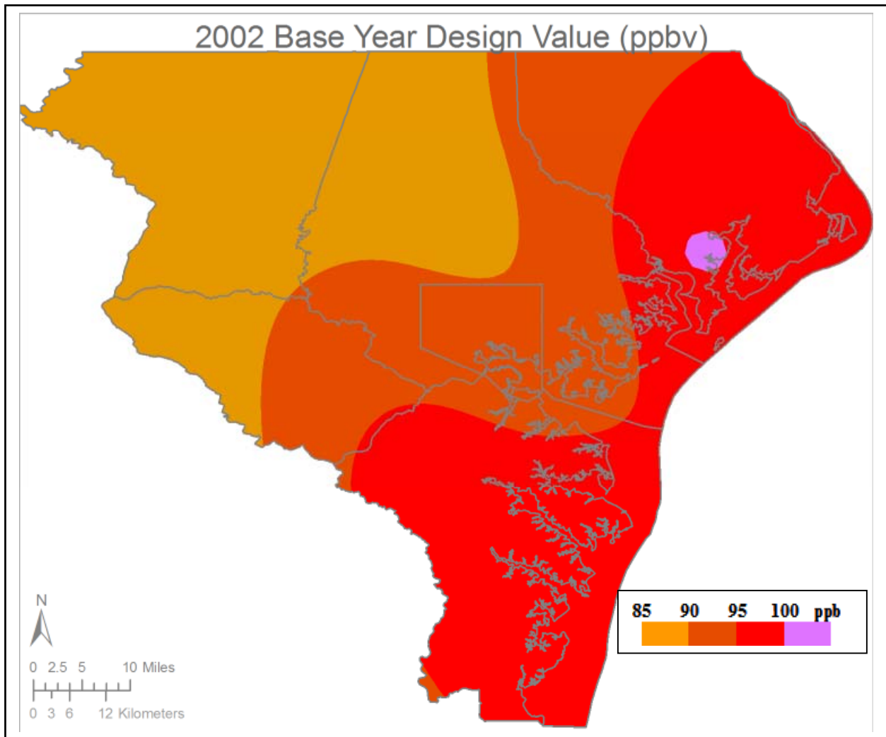
Figure 12-5 Spatially Interpolated Extent of the 8-Hour Ozone Within the Baltimore NAA Using 2002 Base Year Design Values
