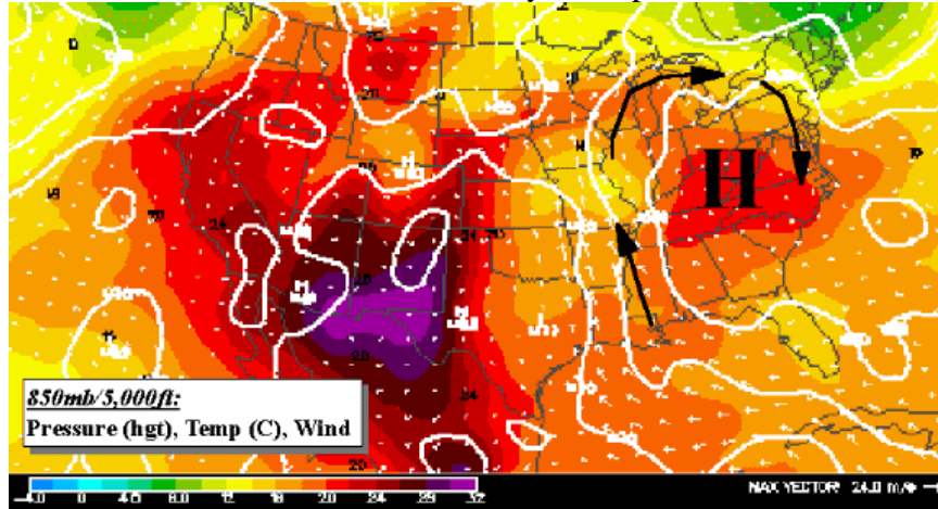
Panel C – Westerly Transport
