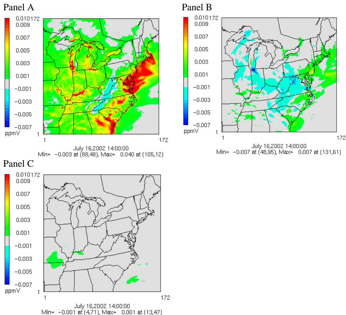
Figure 11.3.3 Differences between standard and revised CMAQ ozone (standard – revised). The standard CMAQ used j\text{NO}_2 values that did not account for aerosols, while the revised CMAQ used j\text{NO}_2 values that did account for aerosols measured for a July 2002 smog and haze episode. These plots are for 9:00 EST at the surface (Panel A), 500m (Panel B), and 3400m (Panel C) AGL.
