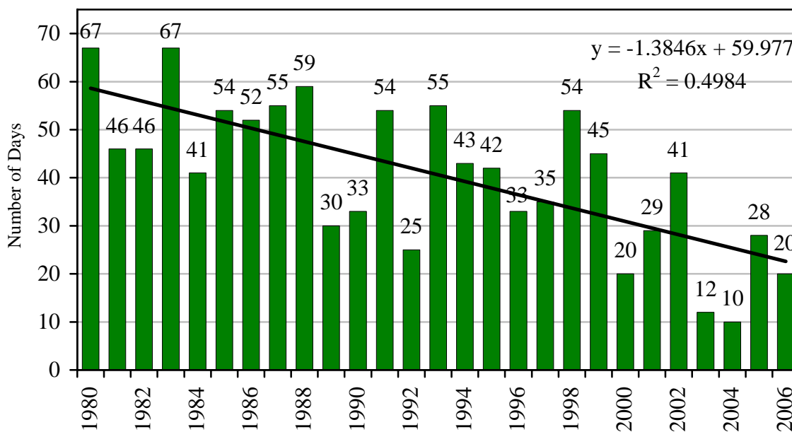
Figure 11.1.3 Trend in 8-hour ozone exceedance days per year for all Maryland sites. The declining trend is an indicator of improving air quality.
