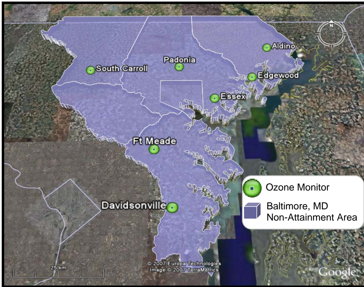
Figure 12-2 Locations of Ozone Monitors in the Baltimore NAA
