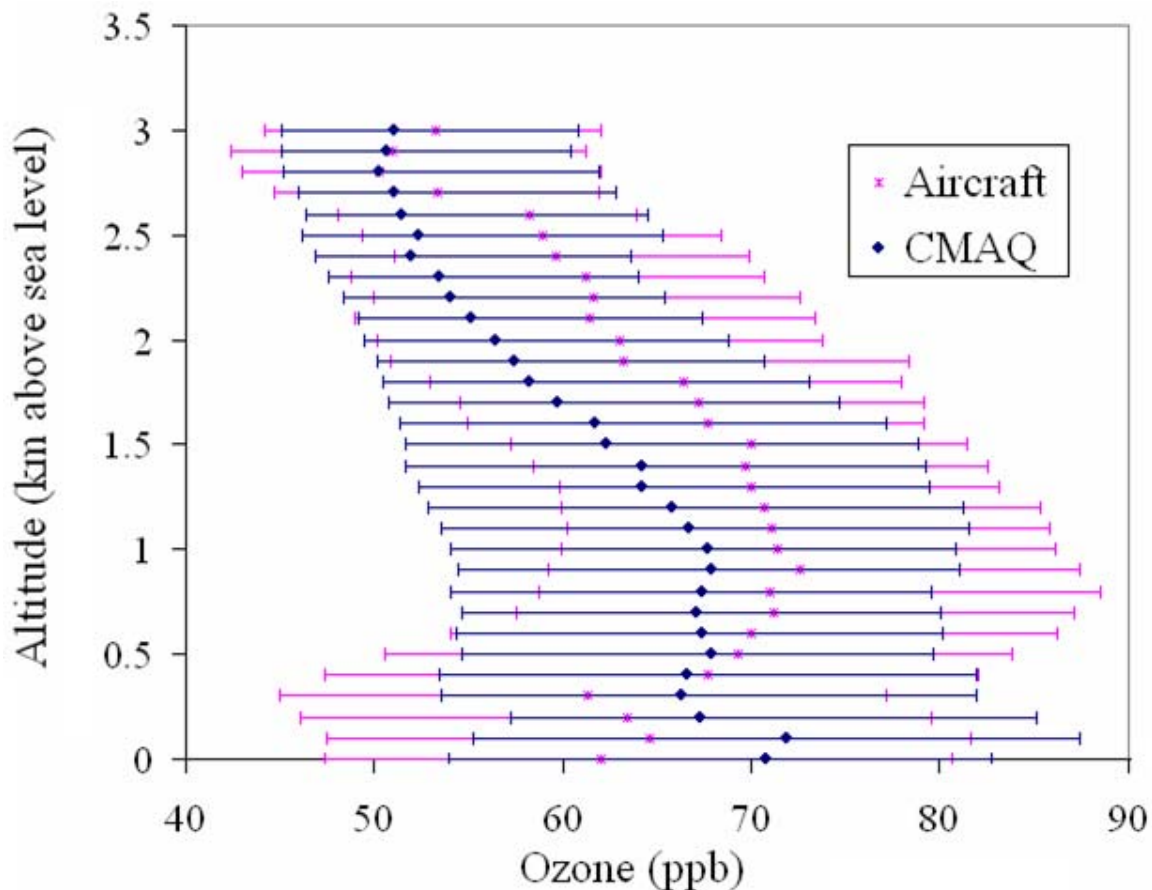
Figure 11.3.1 Median CMAQ and aircraft O 3 profiles from 2002 (June–August, 136 profiles). The ends of the horizontal bars represent the 25 th and 75 th percentiles.
