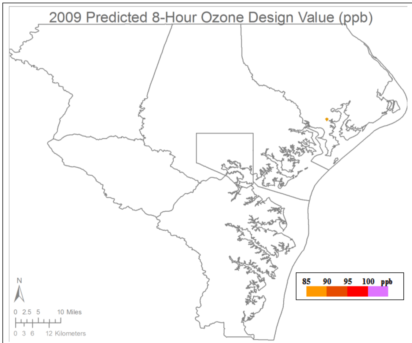
Figure 12-6 Spatially Interpolated Extent of the 8-Hour Ozone Within the Baltimore NAA Using 2009 Predicted Future Year Design Values
