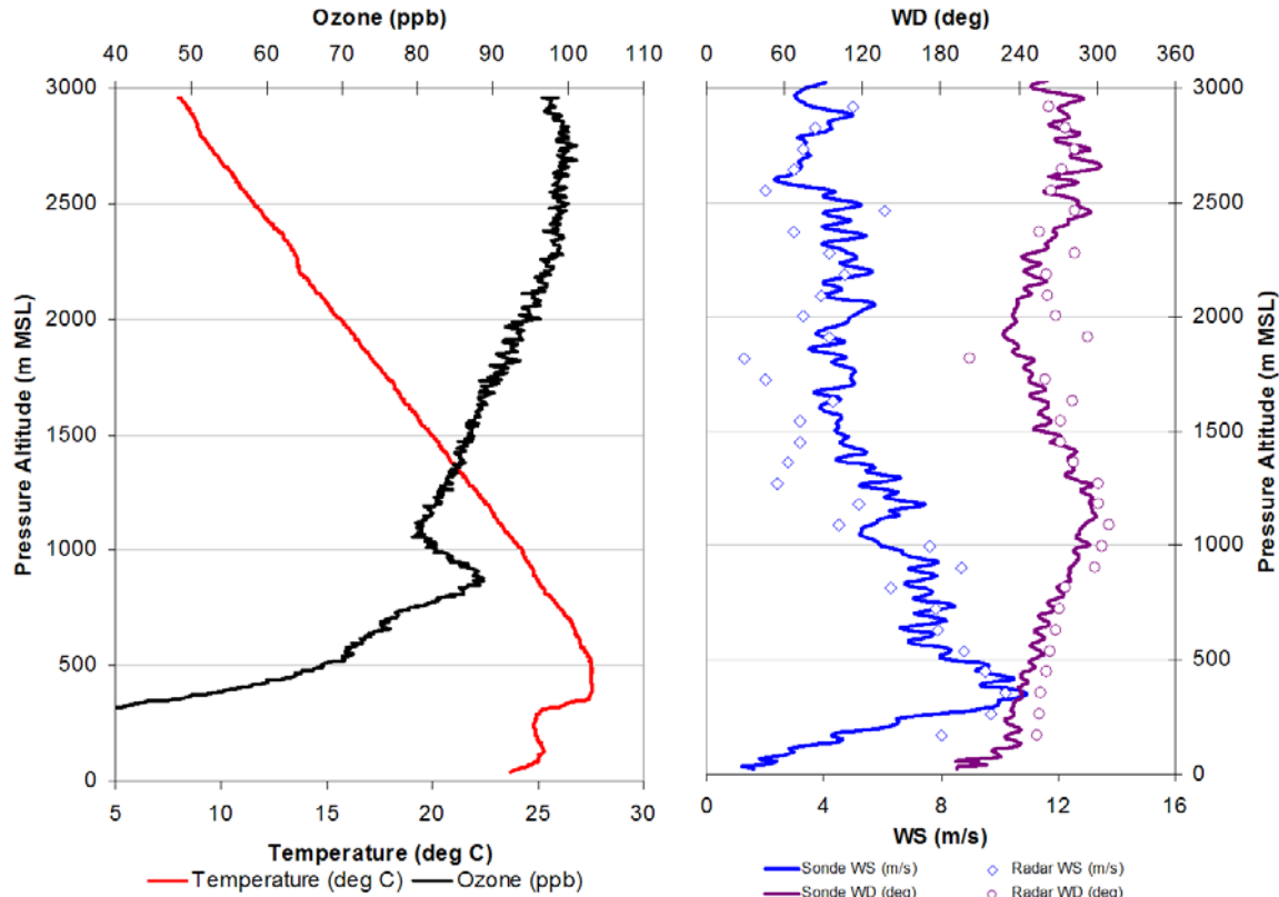
Figure 11.2.9 Ozonesonde balloon data are shown as vertical profiles through the atmosphere. Radar winds are overlaid with the blue and purple data points. Two balloon launches took place on August 5, 2005. A. 3:30 AM EST on August 5, 2005 B. 7:30 AM EST on August 5, 2005
