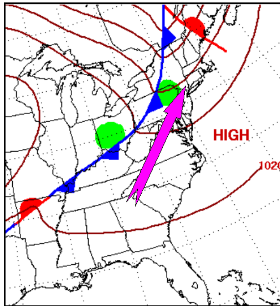
Figure 11.2.7 Synoptic weather analysis from August 5, 2005 at 7:00 AM EST. The pink arrow indicates the theoretical position of the NLLJ.
