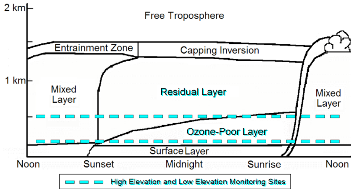
Figure 11.2.2 Diagram of the atmospheric boundary layer. The nocturnal atmosphere stratifies into a residual layer aloft where interstate pollutant transport may be measured.
