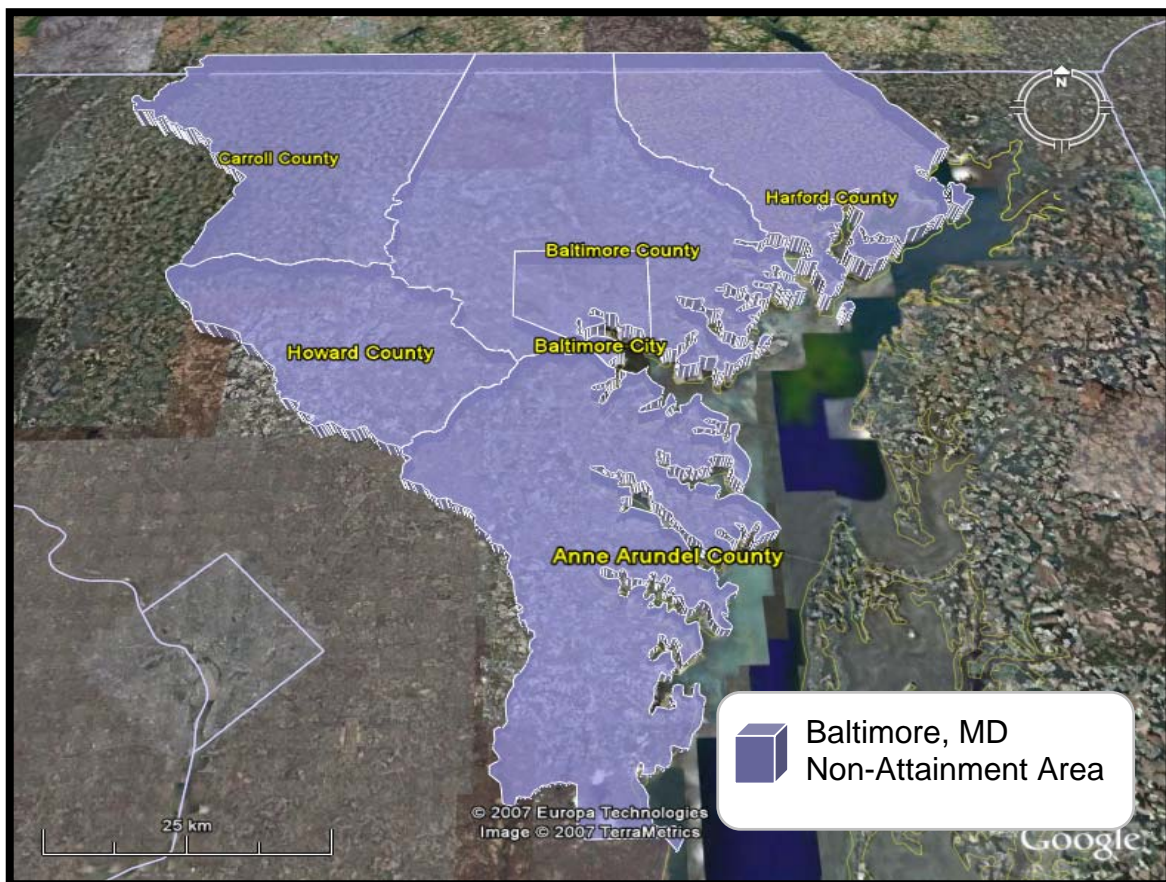
Figure 12-1 8-Hour Ozone Baltimore NAA
