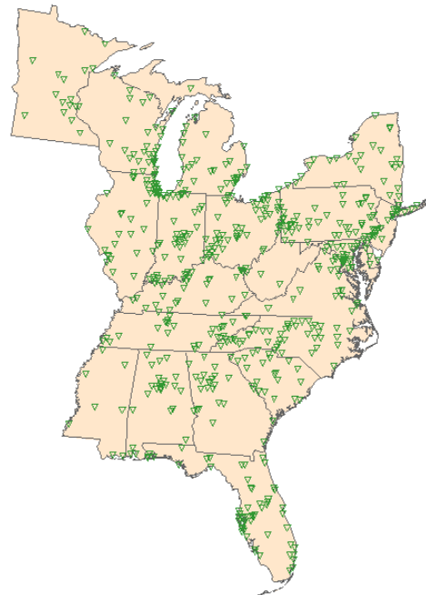
Figure 11.1.1 Maps of the 2006 ozone monitoring sites (blue circles in Panel A and inverted green triangles in Panels B and C). There are 17 ozone monitoring sites in the state of Maryland, a dense network for a relatively small state.
