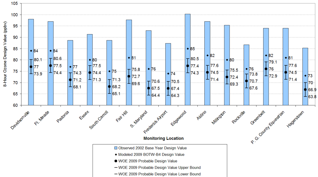
Figure 11.3.5 A graphical depiction of the data from Table 11.3.1, depicting 2002 base year design values (blue columns), modeled 2009 design values (black diamonds), and the WOE probable future year design values along with the upper and lower bounds for those future year values (round circles and associated error bars, respectively). All Maryland monitoring locations are shown. All sites are under the NAAQS for 8-hour ozone.
