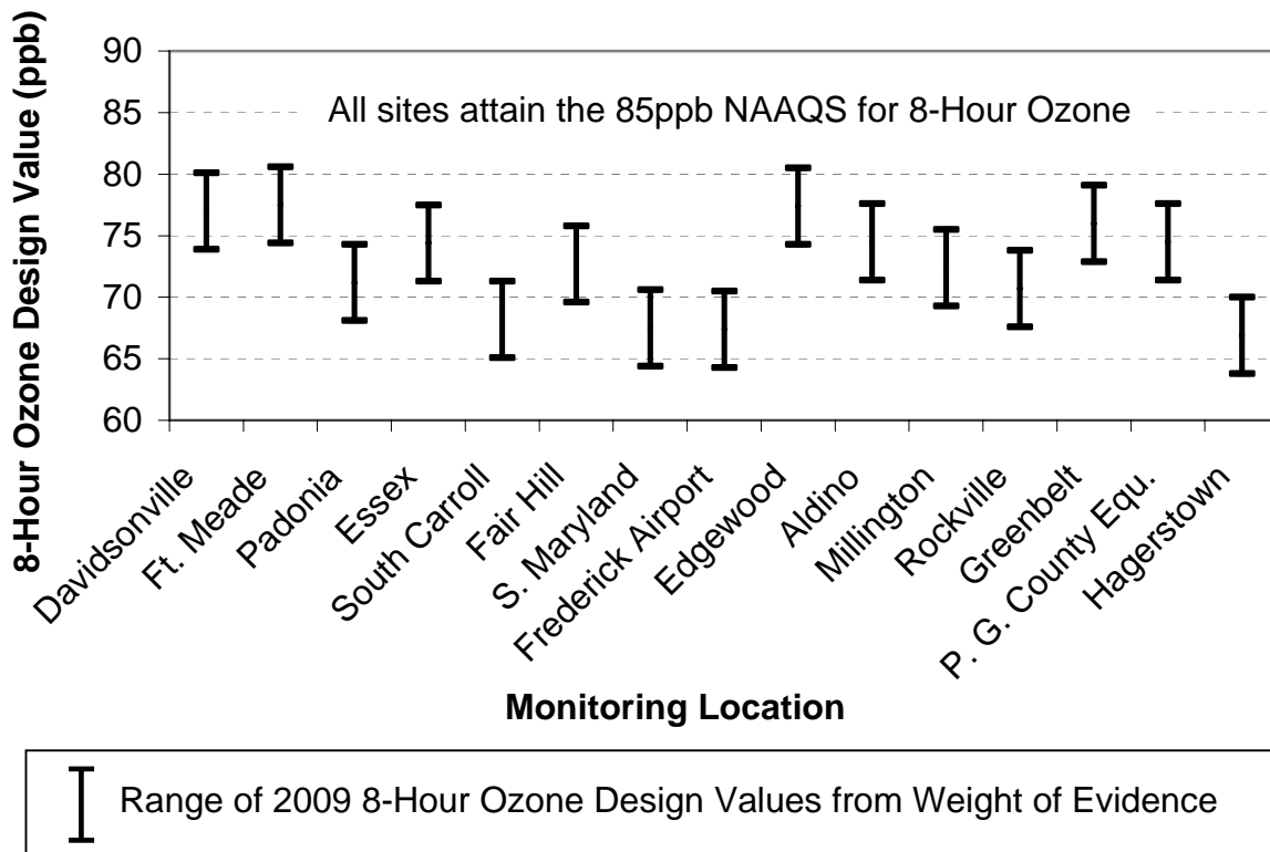
Figure 11.0.1 Range of probable 2009 8-hour ozone design values for all sites in Maryland
