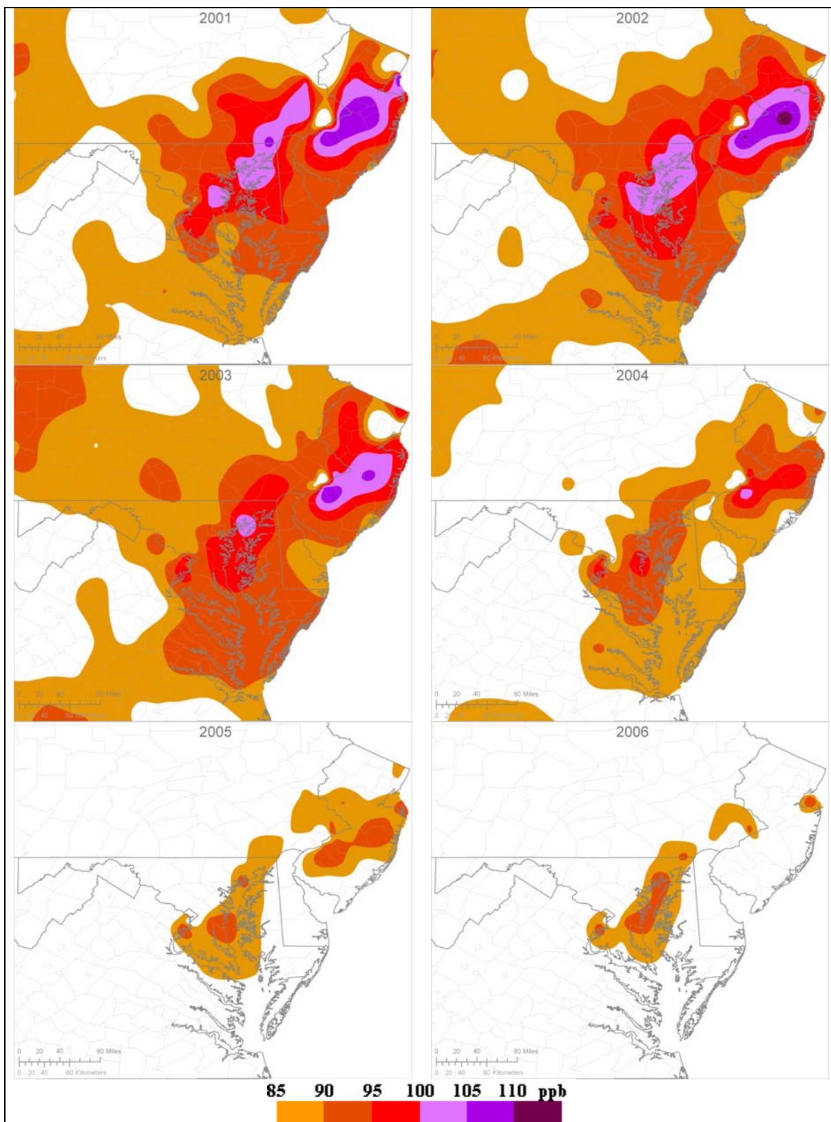
Figure 11.1.6 1995-2006 improving trend exhibited by decreasing spatial extent and magnitude of 8-hour ozone design values \geq 85 ppb.
