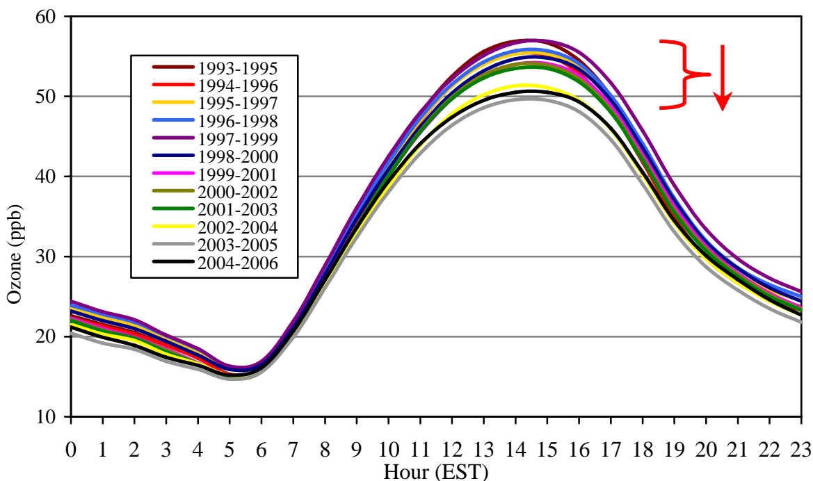
Figure 11.1.5 Trend in diurnal ozone by 3-year rolling averages for all Maryland sites from the summers (April 1 – October 31) of 1993 through 2006. The red brace and arrow indicate improving air quality shown by the decreasing trend of peak mid-day hourly concentrations.
