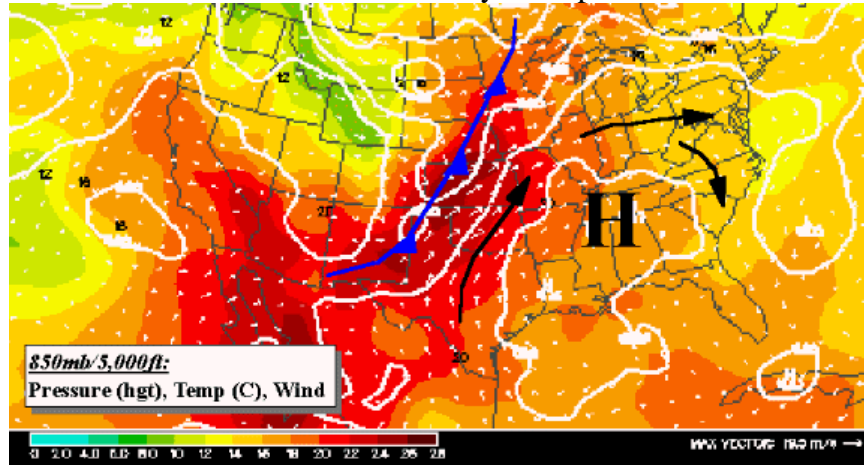
Panel D – Pre-Frontal Transport
