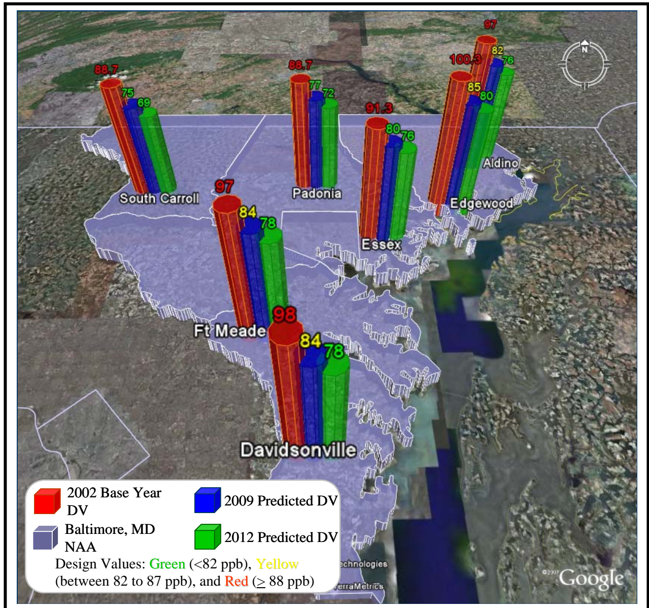
Figure 12-8 Baltimore NAA 8-Hour Ozone Base Year (2002) and Predicted Future Years (2009 and 2012) Design Values
