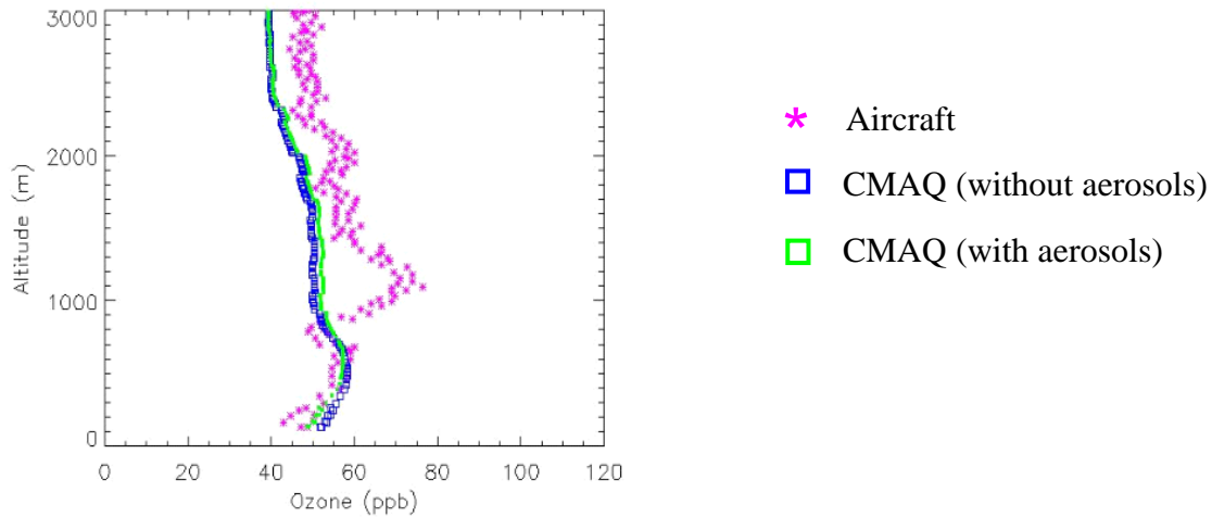
Figure 11.3.3 Ozone profiles from the aircraft (pink stars), CMAQ using standard j\text{NO}_2 values (without aerosols, and shown in blue open squares), and CMAQ using revised j\text{NO}_2 values (with aerosols, shown in green closed squares) for July 17, 2002.
