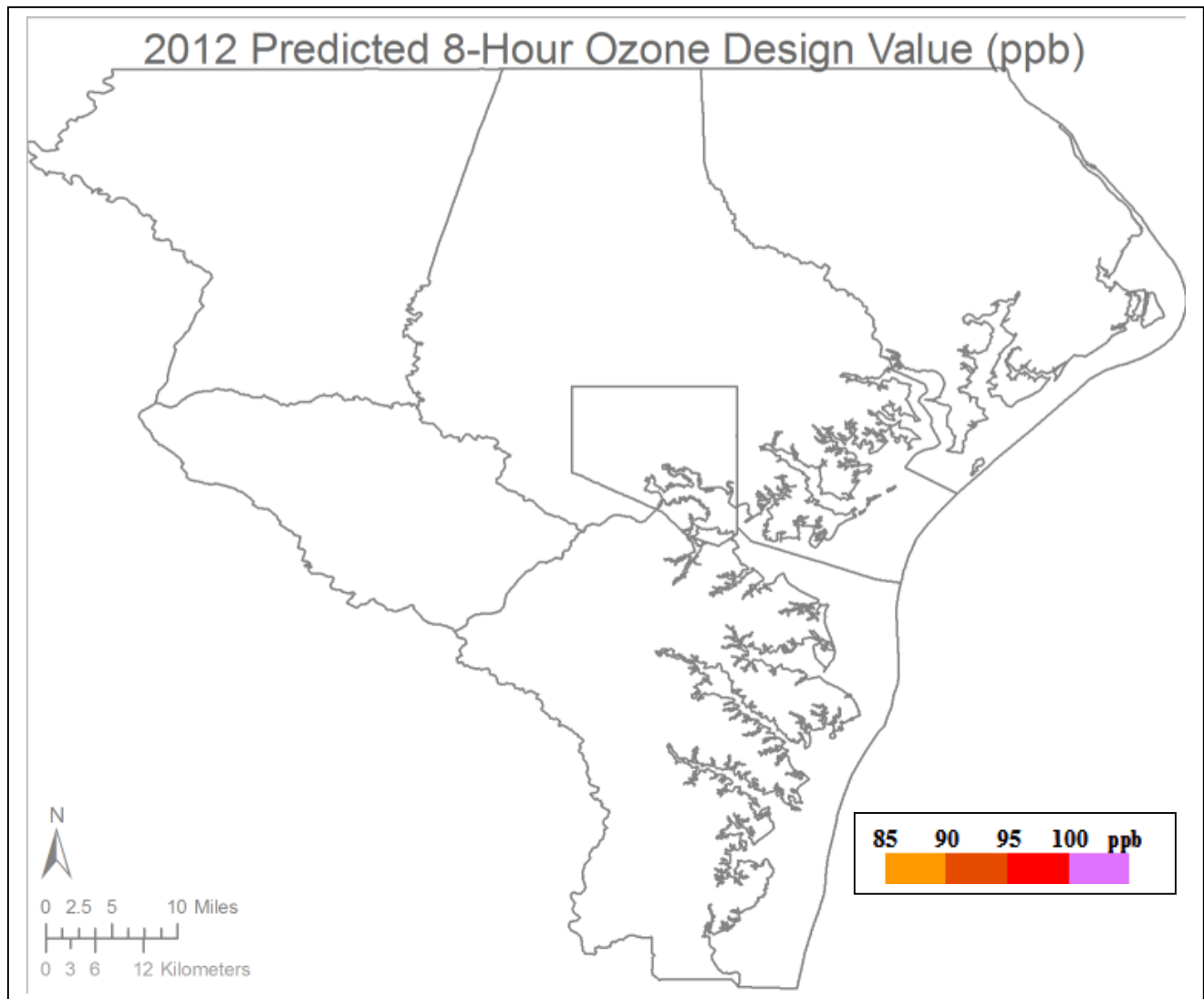
Figure 12-7 Spatially Interpolated Extent of the 8-Hour Ozone Within the Baltimore NAA Using 2012 Predicted Future Year Design Values
