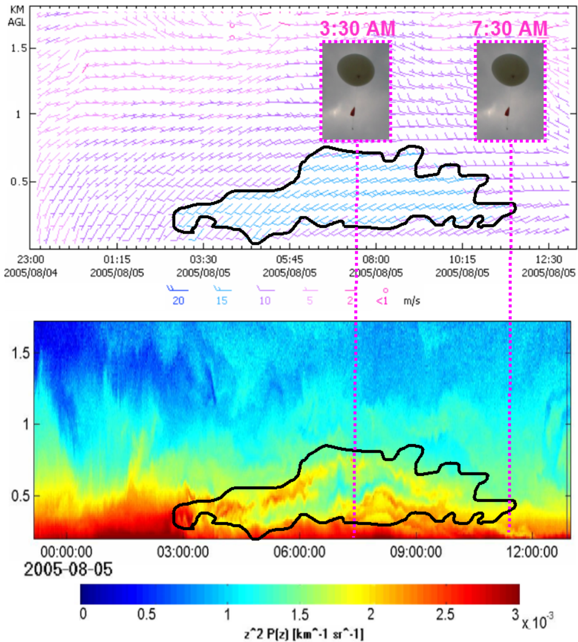
Figure 11.2.8 The top portion of the time-height plot depicts winds from the RADAR at Beltsville, Maryland. The bottom portion of the time-height plot depicts aerosol scattering from the LIDAR at Catonsville, Maryland. The black, amoeba-shaped, line is drawn around the portion of the RADAR data that fits the stereotypical characteristics of a NLLJ. The same black shape was also overlaid on the LIDAR data. The timing of two ozonesonde balloon launches from Beltsville, Maryland are also overlaid in pink, dashed lines at their respective launch times.
