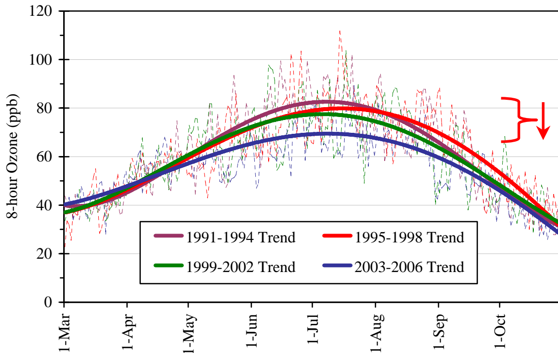
Figure 11.1.4 Trends in average daily peak 8-hour ozone for all Maryland sites binned by four-year periods. The red brace and arrow indicate improving air quality shown by the decreasing trend of average daily peak 8-hour ozone. Each trend line is fourth order.
