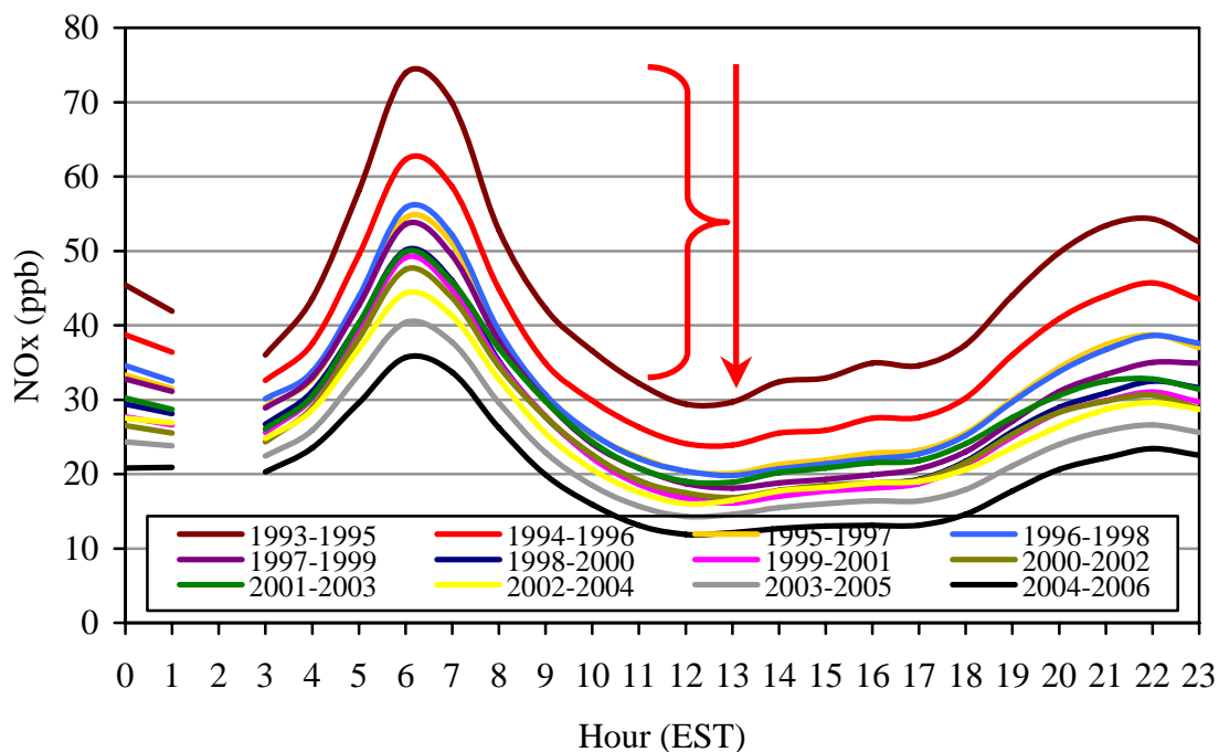
Figure 11.1.8 Trend in diurnal \text{NO}_x by 3-year rolling averages for all sites in Maryland from the summers (April 1 – October 31) of 1993 through 2006. The red brace and arrow indicate improving air quality shown by the decreasing trend of peak hourly concentrations. Instrument calibration occurs during the data gap at 2:00 AM EST.
