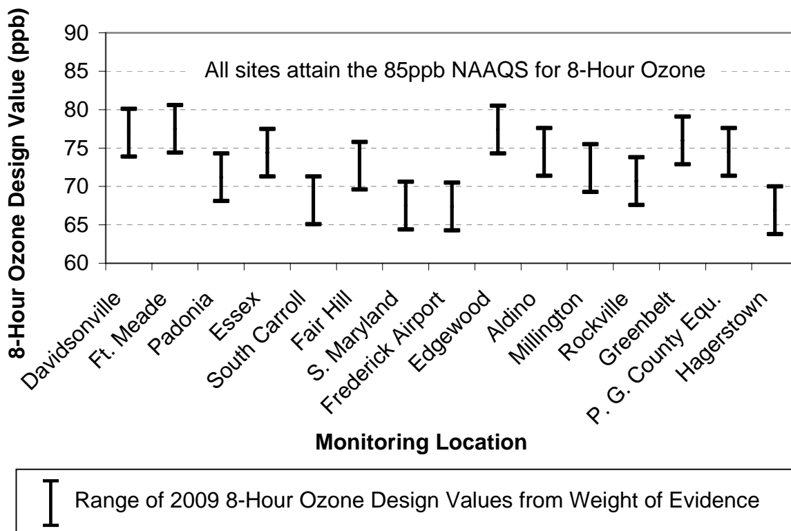
Figure 11.3.4 2009 probable ranges for design values in Maryland. The lower end of each bar represents the lower bound of the most likely future year design value, while the upper end of each bar represents an upper bound.
