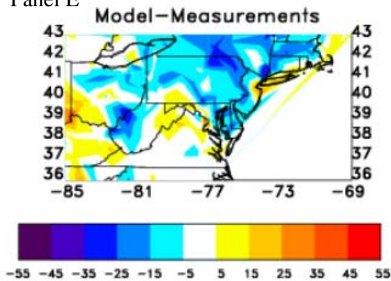
Figure 11.3.2 Tuesday, June 25, 2002, 10:00 AM EST, Winchester, VA. Case Study A. 24-hour HYSPLIT back trajectories terminating over Winchester, VA. Blue = 500m, Green = 1000m, Red = 1500m B. Aircraft (pink stars) and CMAQ (blue diamonds) ozone profiles. C. OTR surface ozone monitor data. D. 2002 base B1 CMAQ simulation averaged for OTR monitor locations. E. Difference plot. Negative values indicate model under-prediction.
