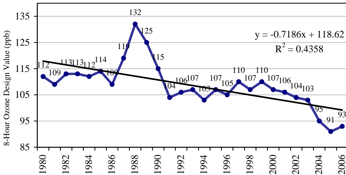
Figure 11.1.2 Trend in 8-hour ozone design values per year for all Maryland sites. The declining trend is a sign of improving air quality.
