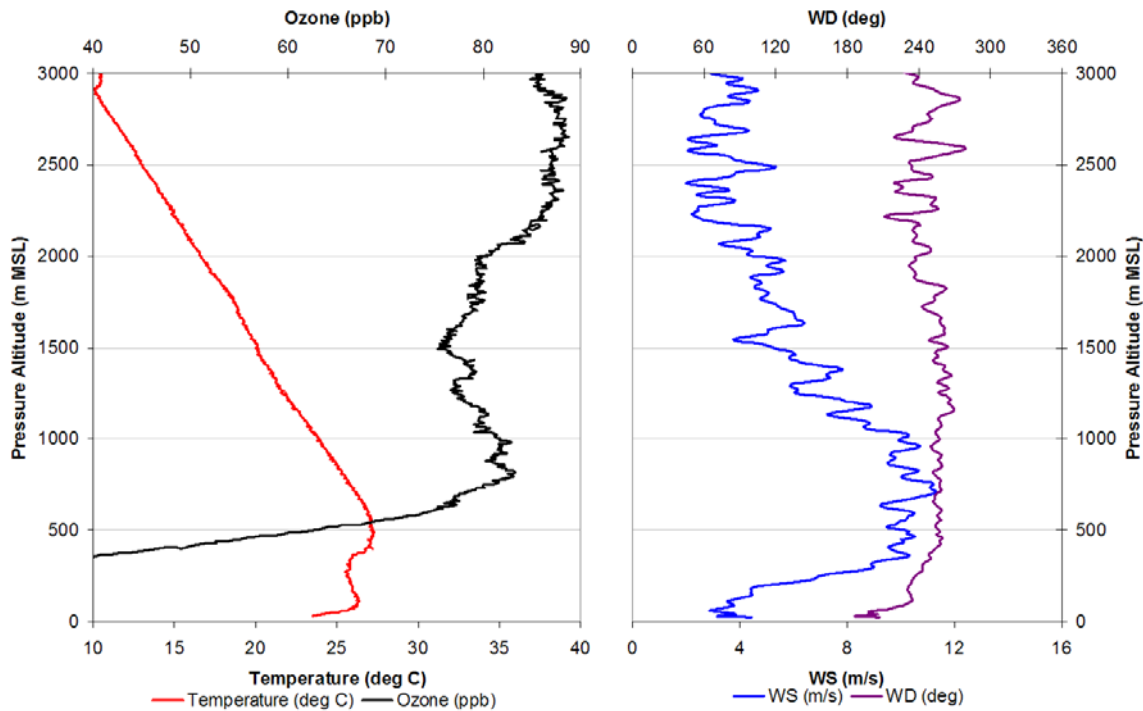
Figure 11.2.5 Ozonesonde balloon launch at 6:00 AM EST on August 15, 2005 from Beltsville, Maryland. Ozone is in black, temperature is in red, wind speed is in blue, and wind direction is in purple.
