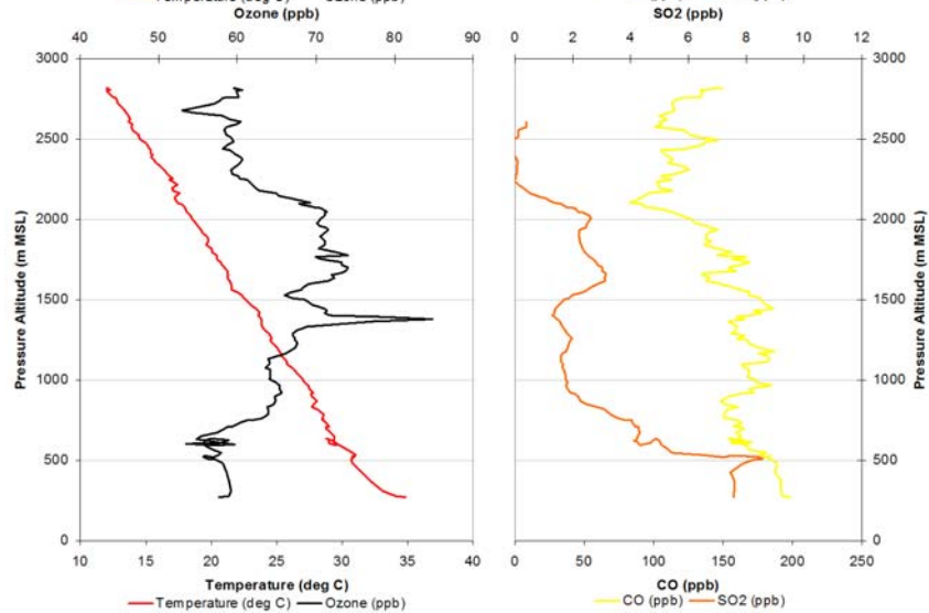
Figure 11.2.6 Aircraft spirals on August 15, 2005. Ozone is in black, temperature is in red, SO2 is in orange, and CO is in yellow.
