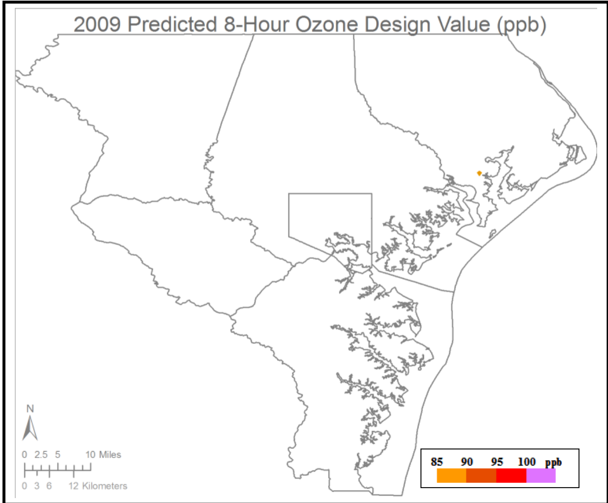
Figure 12-4 Spatially Interpolated Extent of the 8-Hour Ozone in the Baltimore NAA Using Predicted 2009 Design Values
