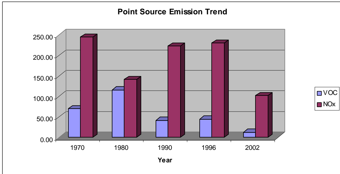
Figure 3.1 Point Source Emission Trends in Tons Per Day*
