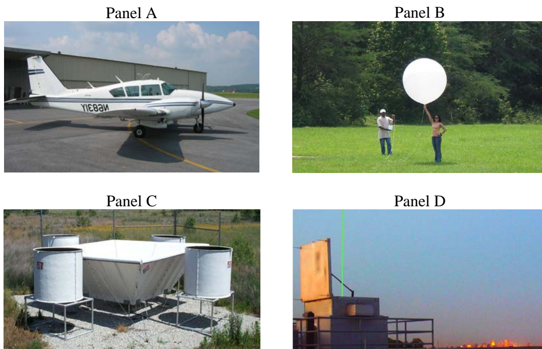
Figure 11.1.9 Supplemental atmospheric profiling initiatives supported by MDE. A. Aircraft, B. Ozonesonde Balloon, C. RADAR, D. LIDAR
