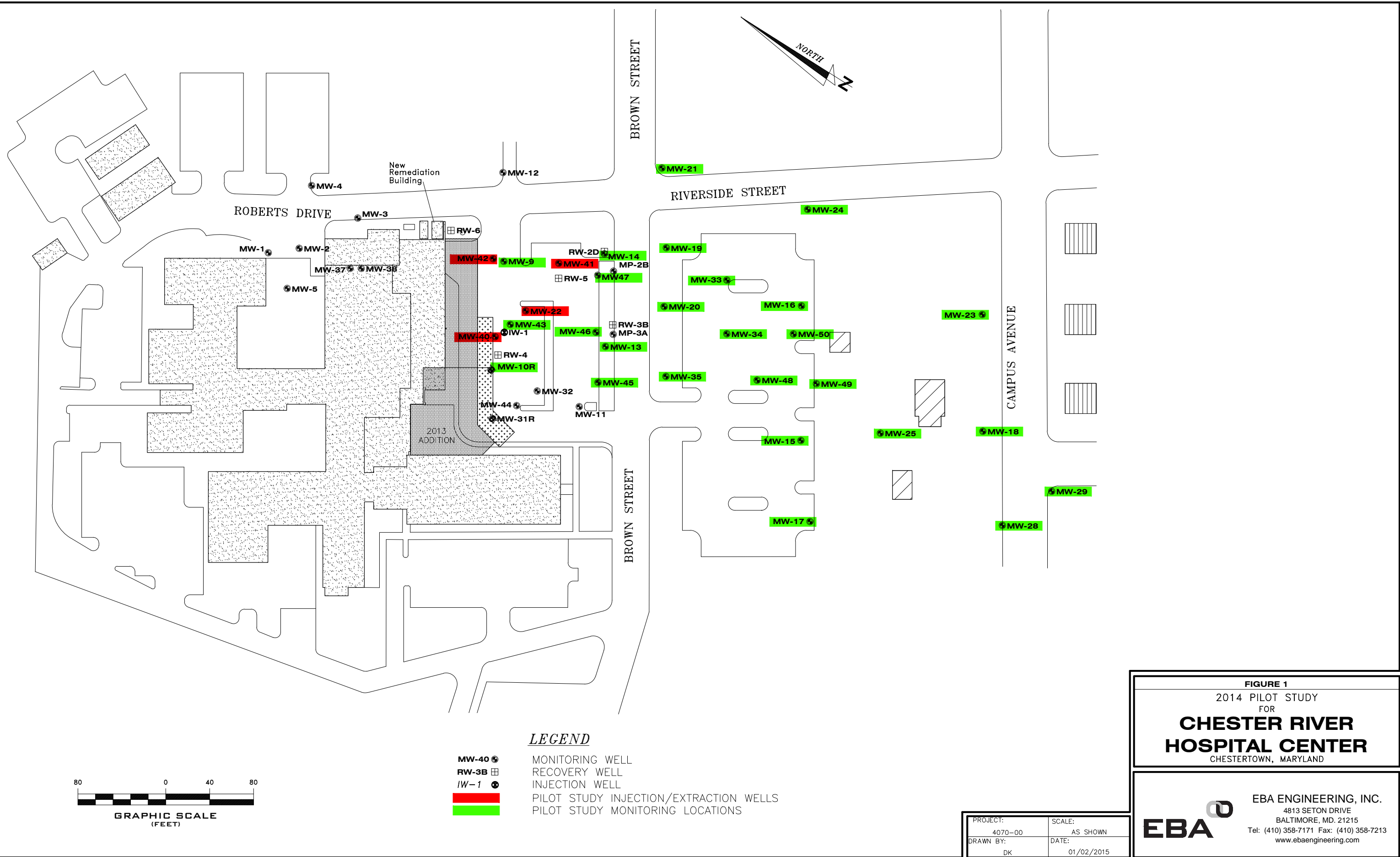
Appendix D Figure 1- Overview of Pilot Study Injection/Extraction Wells and Pilot Study Monitoring Wells
