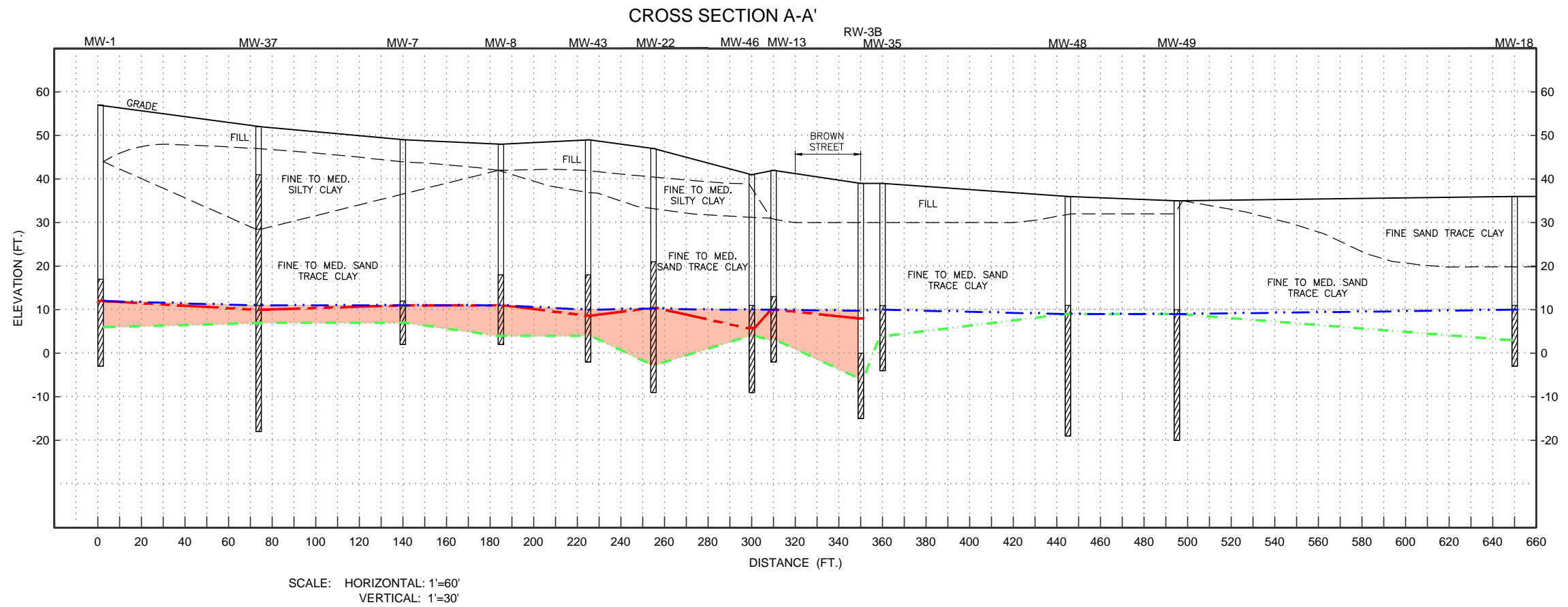
FIGURE 2 CROSS SECTION A-A' FOR CHESTER RIVER HOSPITAL CENTER CHESTERTOWN, MARYLAND
