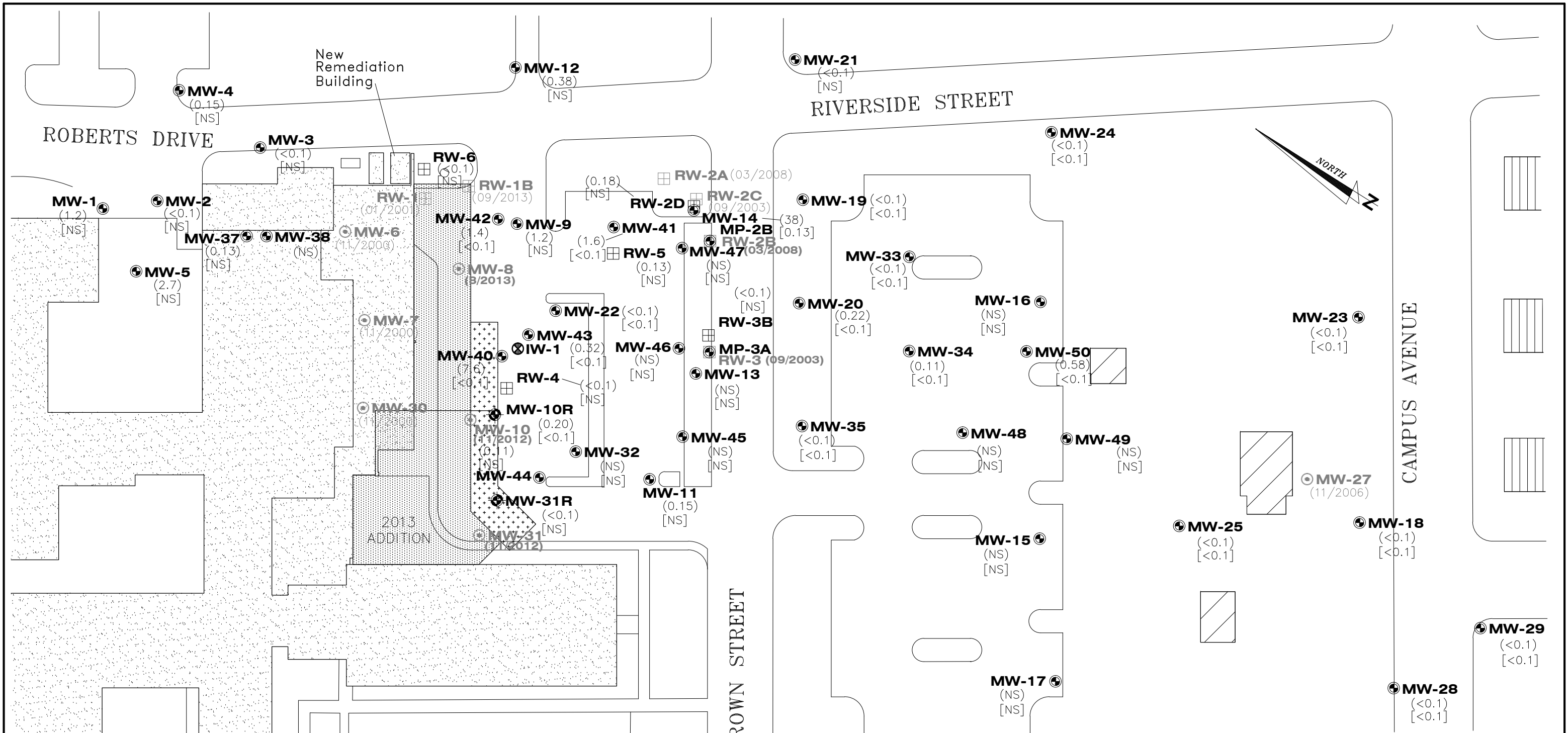
FIGURE 4D DISSOLVED TPH-DRO & TPH-GRO CONCENTRATION MAP FOR CHESTER RIVER HOSPITAL CENTER CHESTERTOWN, MARYLAND
